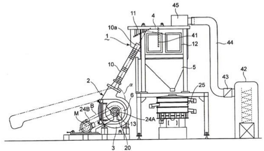
Microsizer component
